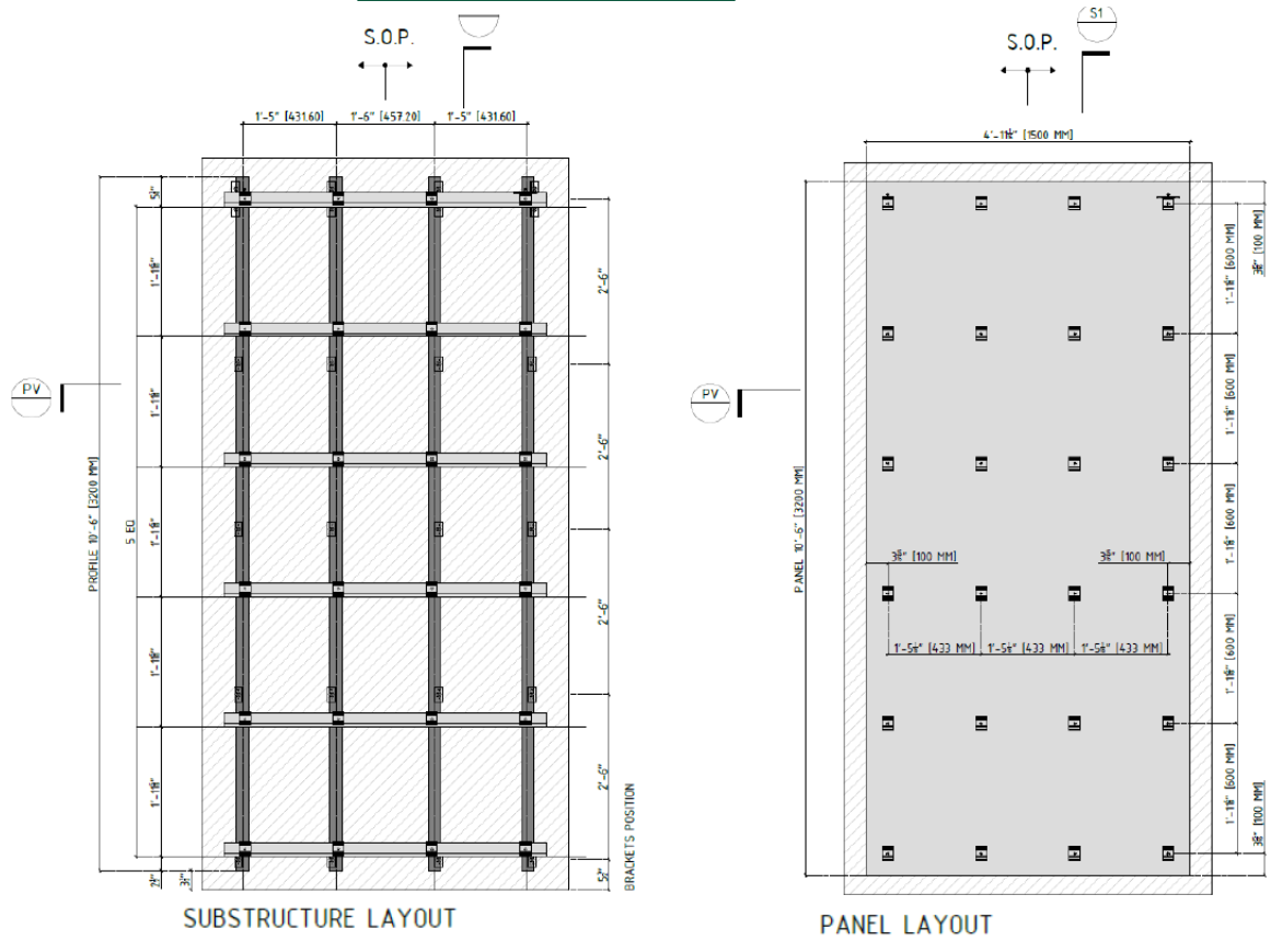
FIGURE 3 – XTONE SUBSTRUCTURE AND PANEL LAYOUT
