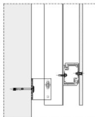
Section View Bottom of System
